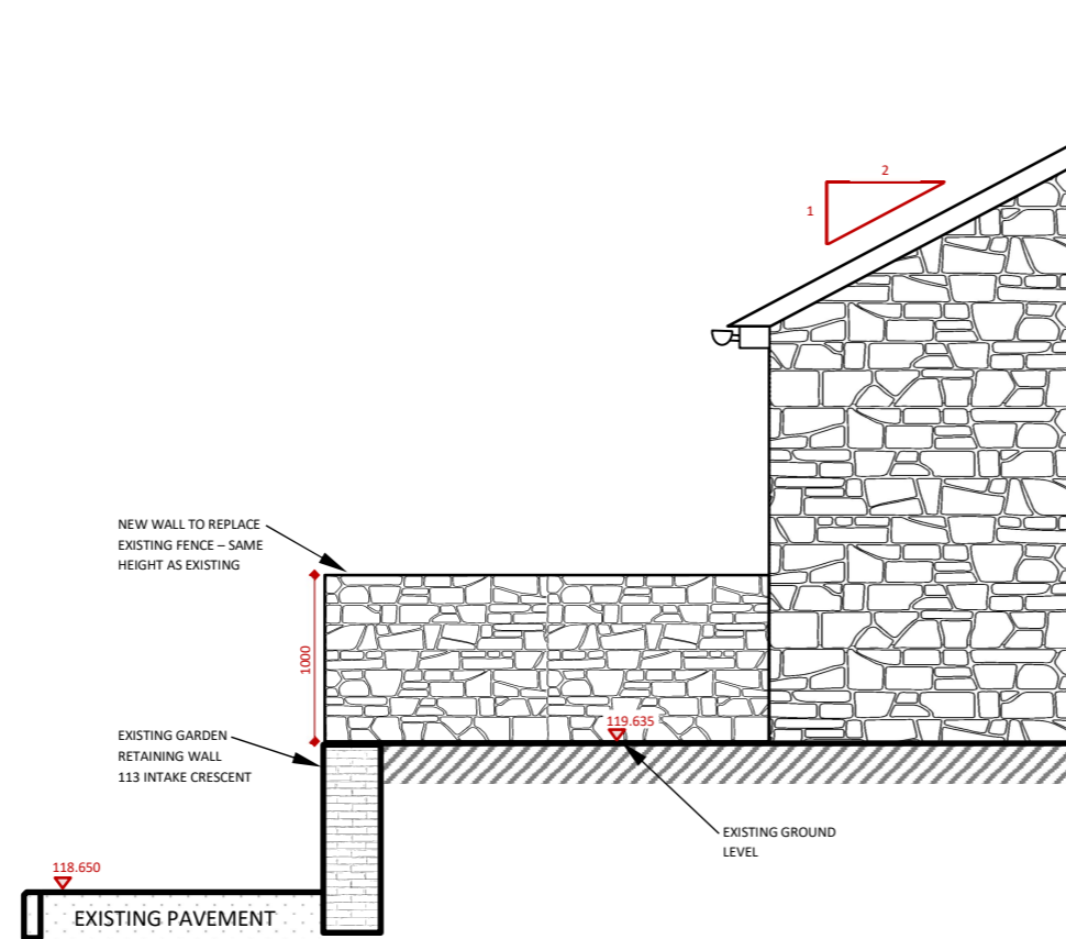
WEST ELEVATION
