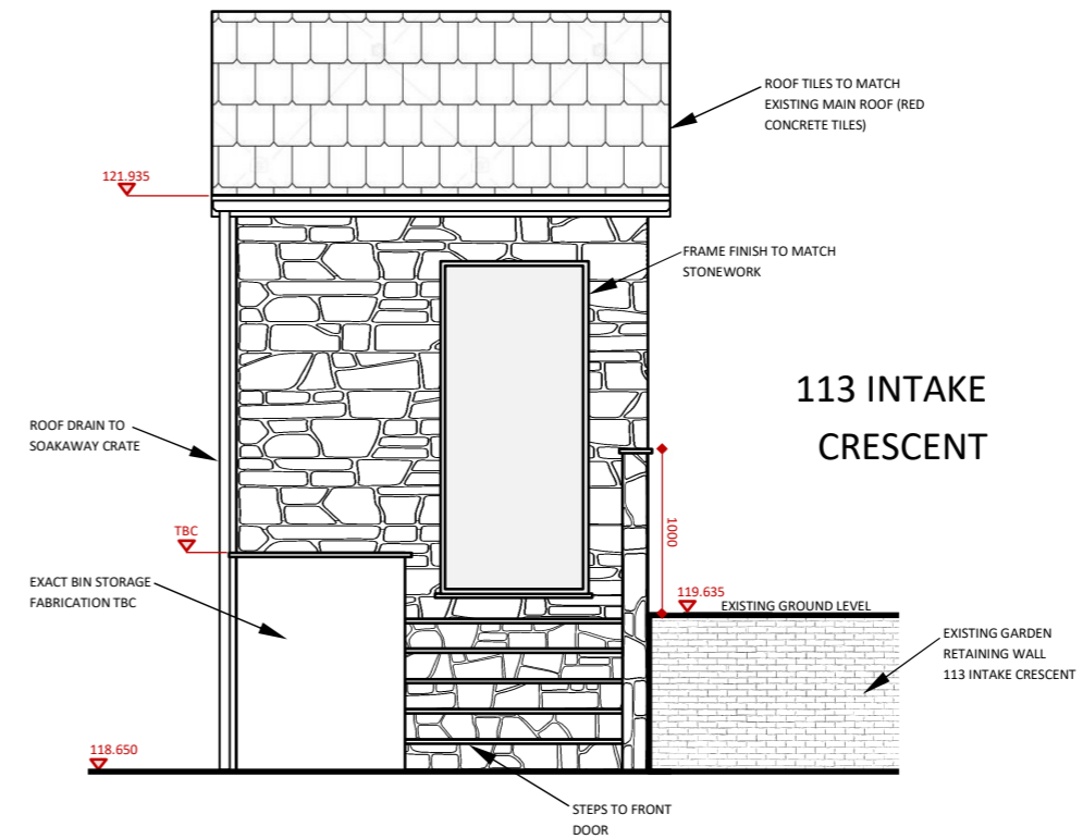
NORTH ELEVATION
