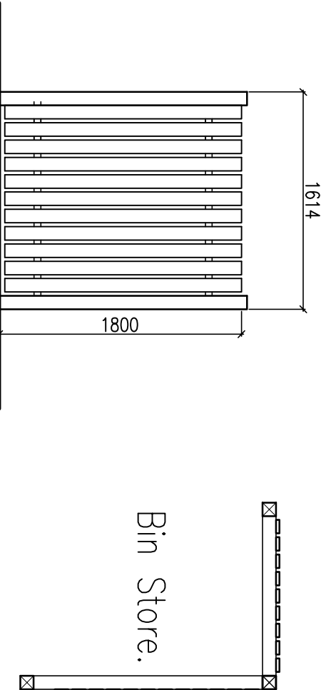
Elevations. Plan.
