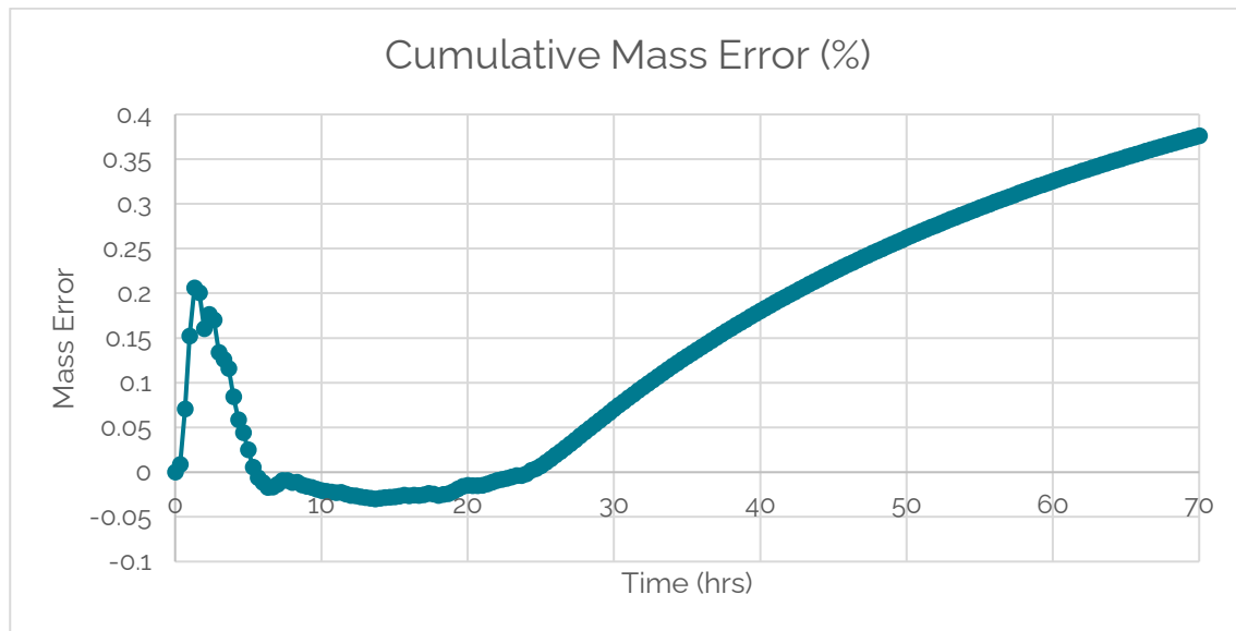
Figure 24. Cumulative 1D Mass Error (Baseline Scenario, 1% AEP + Central CC Event)
