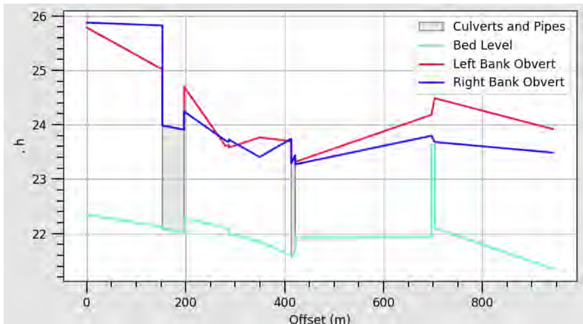
Figure 8. Highgate Lane Dike Modelled Long Section
