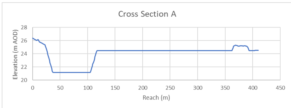
Figure 31. Cross Section A - FCA and Zone 1 Plot Level
