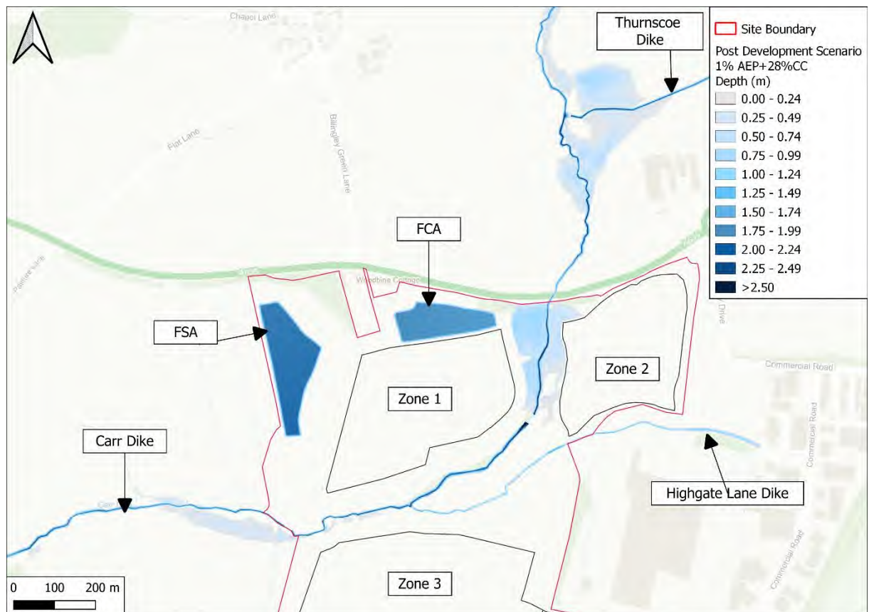
Figure 35: Maximum Extent and Flood Depth for the Post-Development Scenario – 1% AEP plus 'Central' Climate Change
