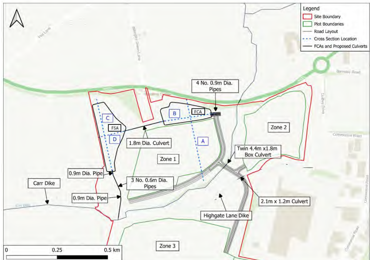
Figure 30. Proposed Development and Mitigation
