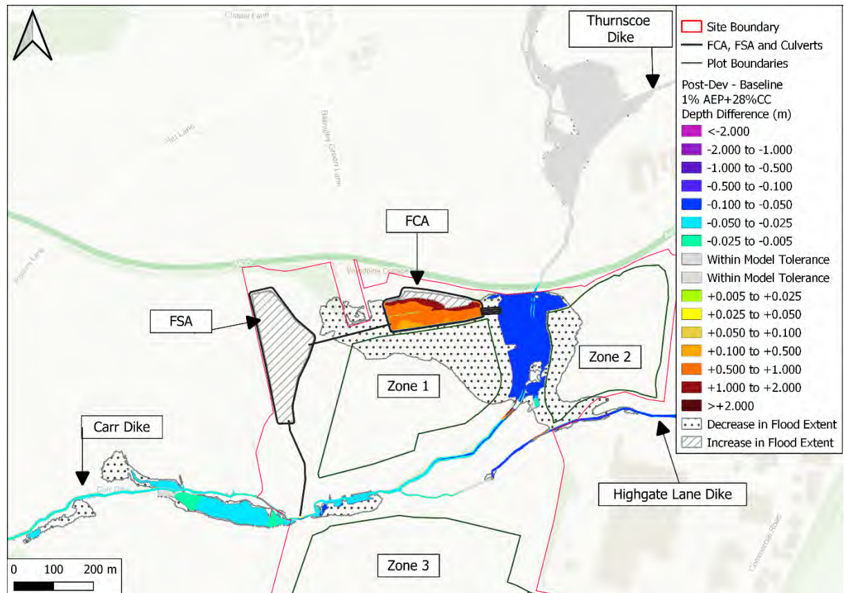
Figure 36. Level Comparison between Post Development & Baseline Scenario - 1% AEP plus 'Central' Climate Change
