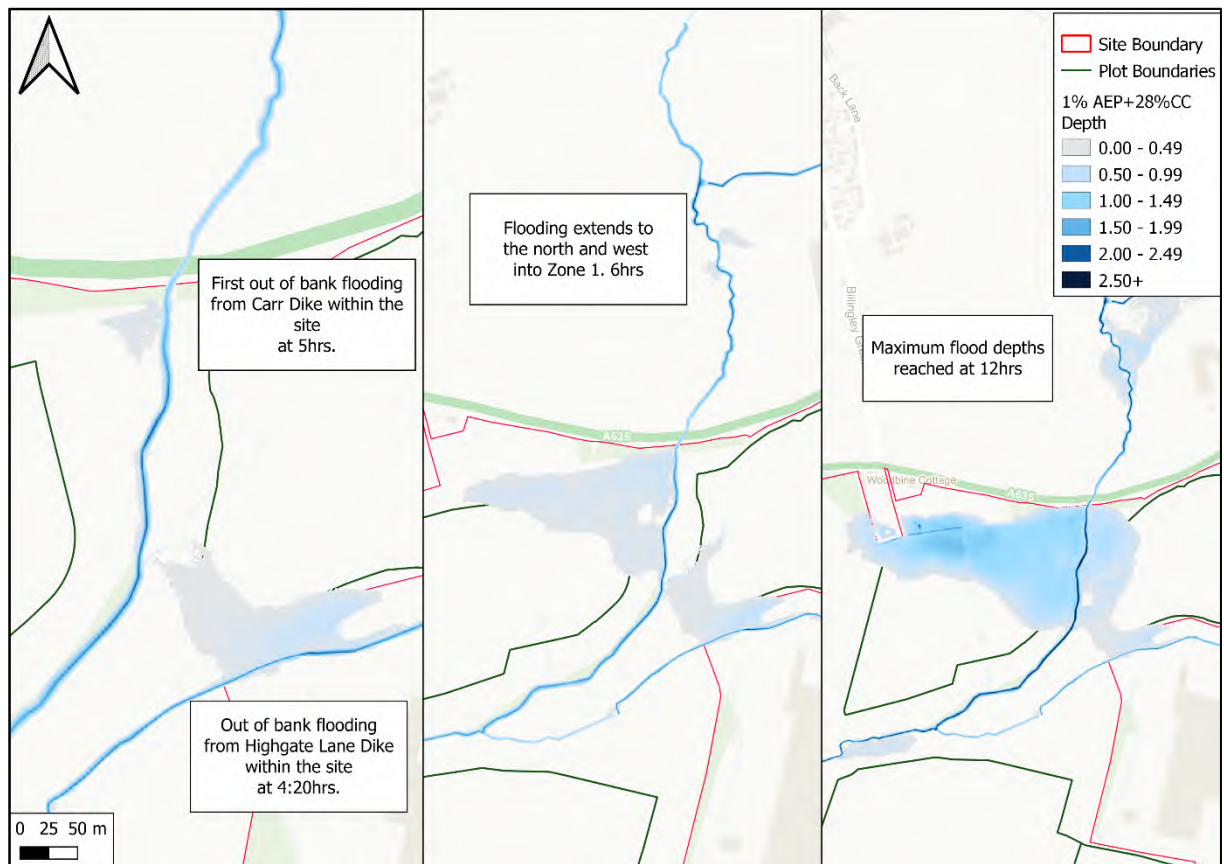
Figure 20. Flood Mechanism in the Baseline Scenario for the Carr and Highgate Lane Dike – 1% AEP plus 'Central' Climate Change
