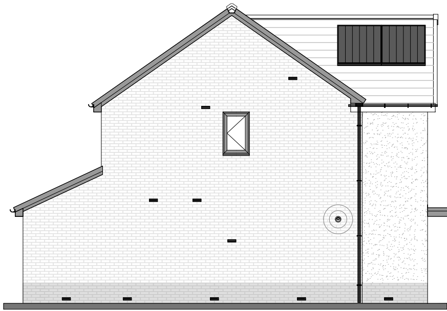
LEFT ELEVATION
