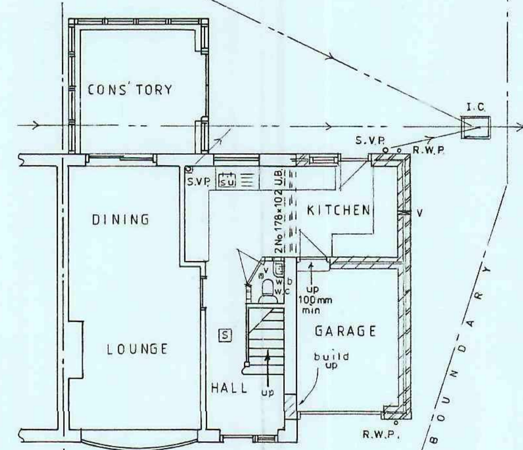
PROPOSED G.F. PLAN
