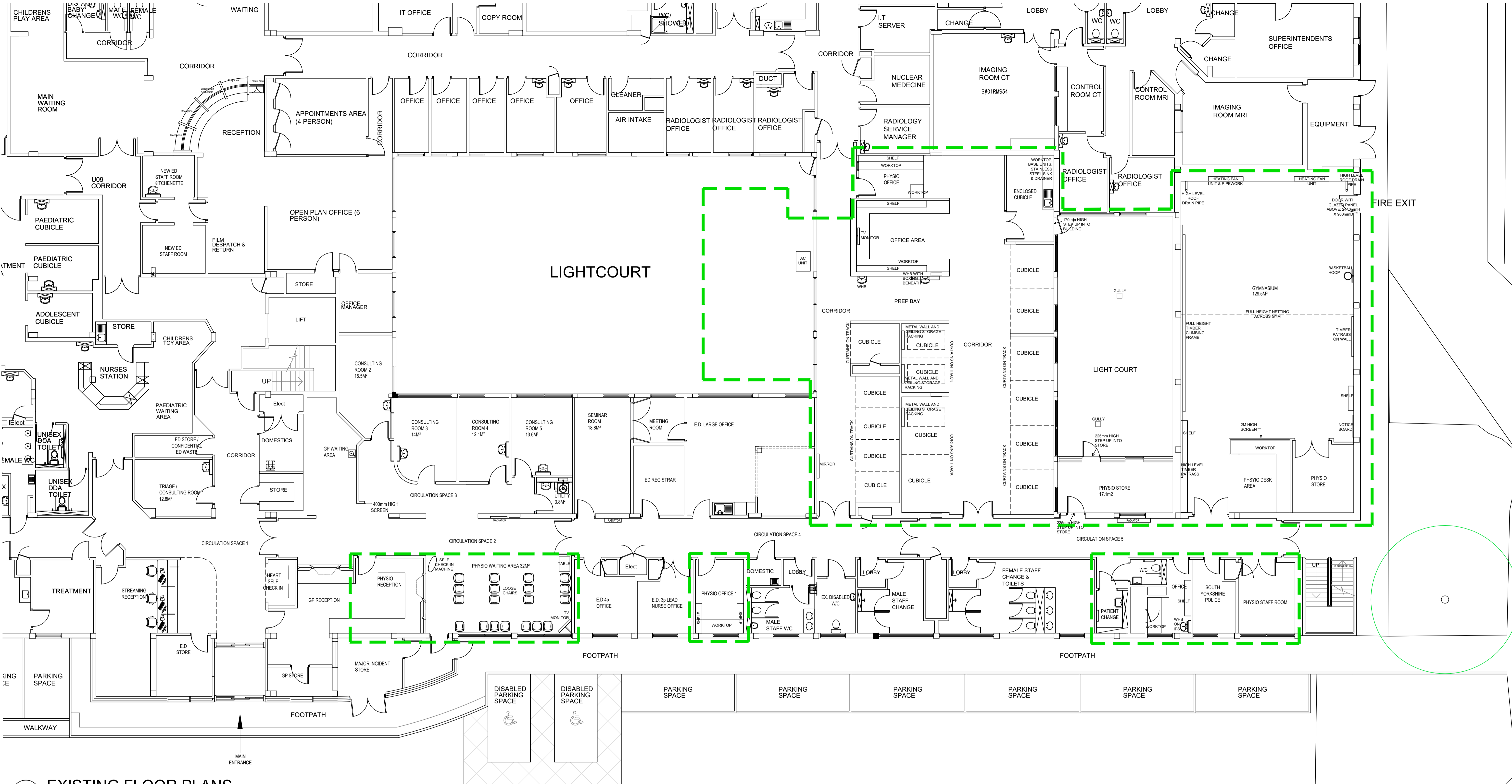
EXISTING FLOOR PLANS 1:100
