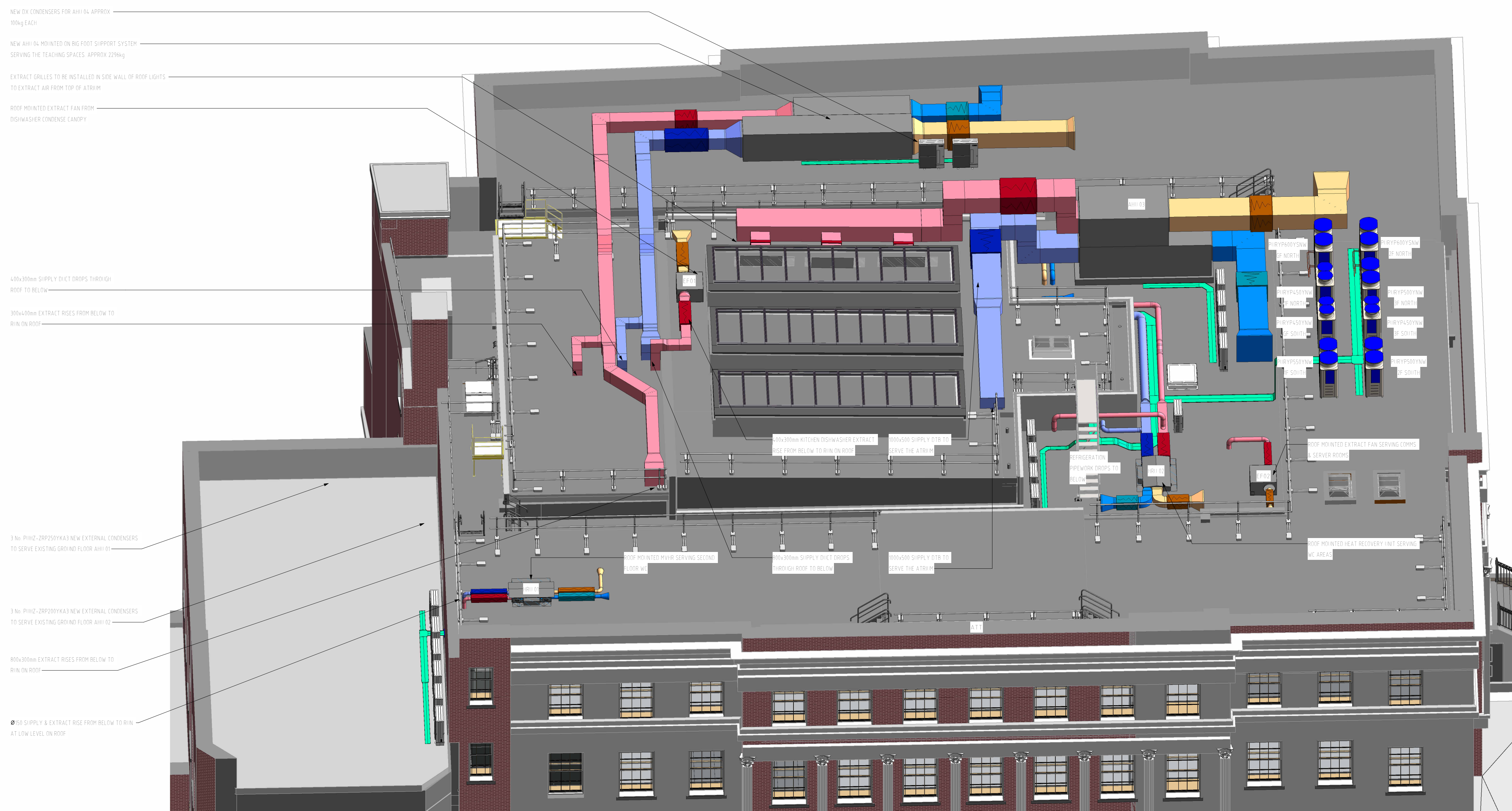
2 ROOF PLANT AREA LAYOUT - 3D VIEW
