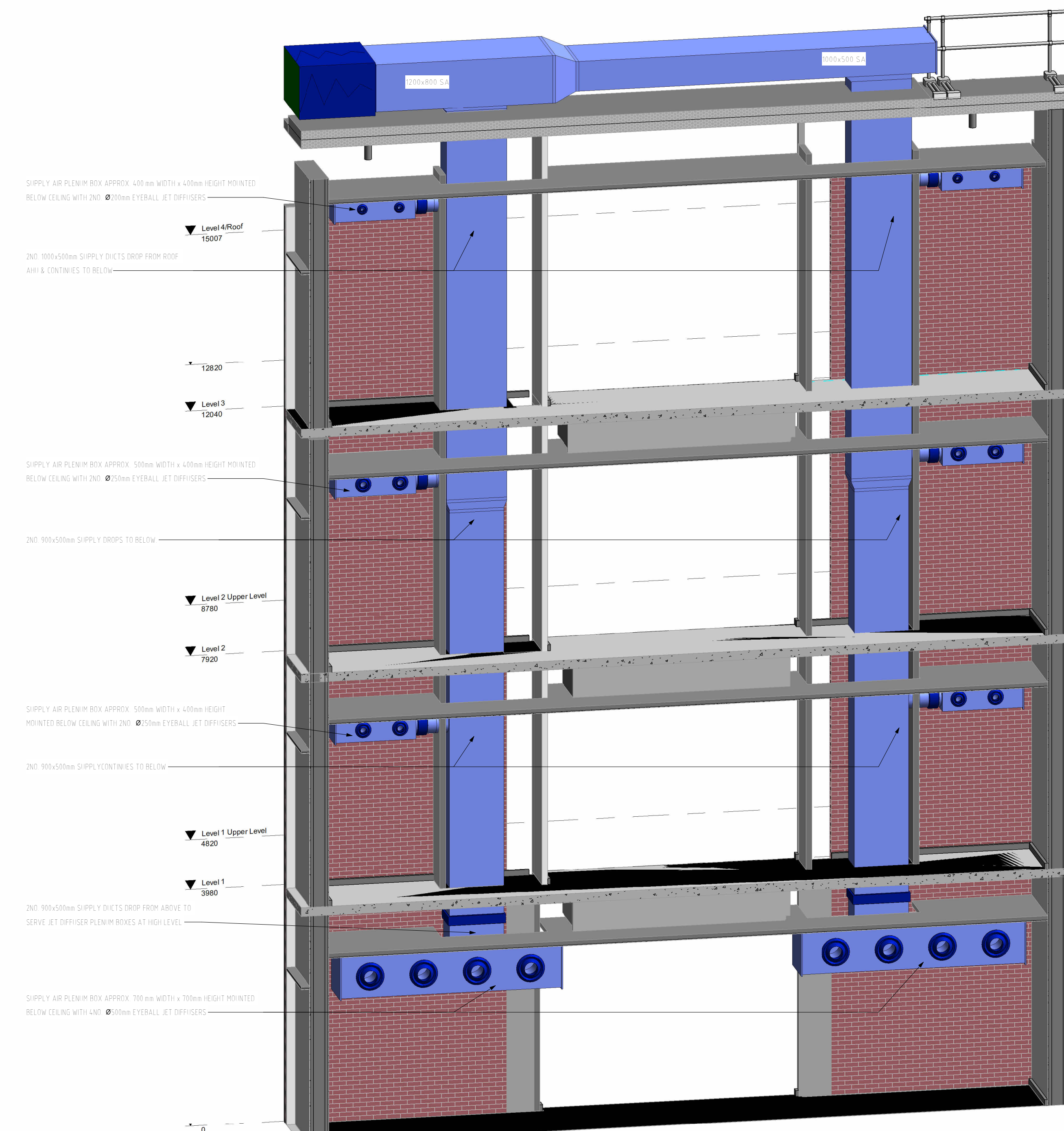
3 AHU 03 SERVING ATRIUM - 3D VIEW
