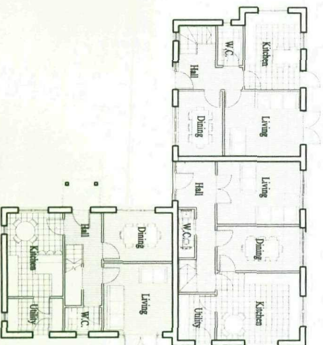
Ground Floor Plan House Type 11 3 Dwellings @ 953, 1365 & 1180 sqft
