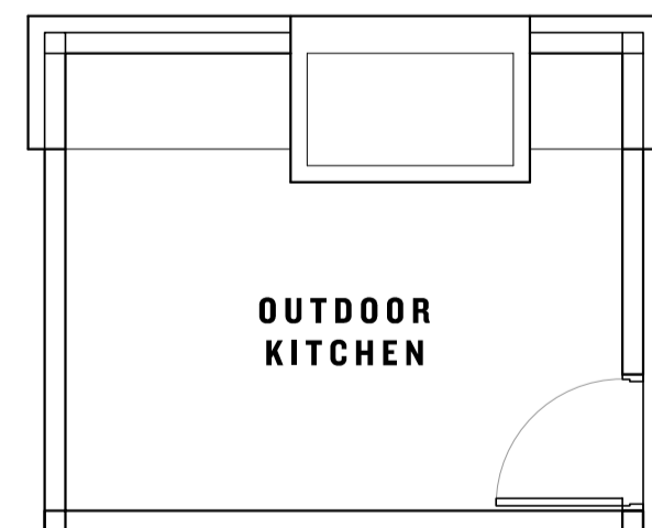
EXISTING HUT FLOOR PLAN Scale - 1: 50 @ A1
