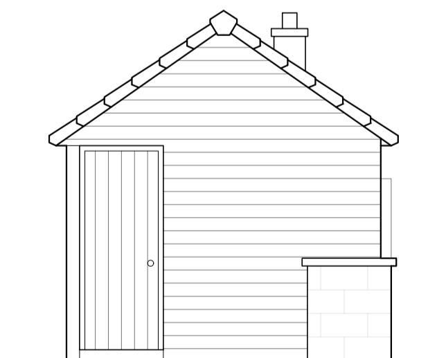
EXISTING HUT FRONT ELEVATION (EAST) Scale - 1: 50 @ A1
