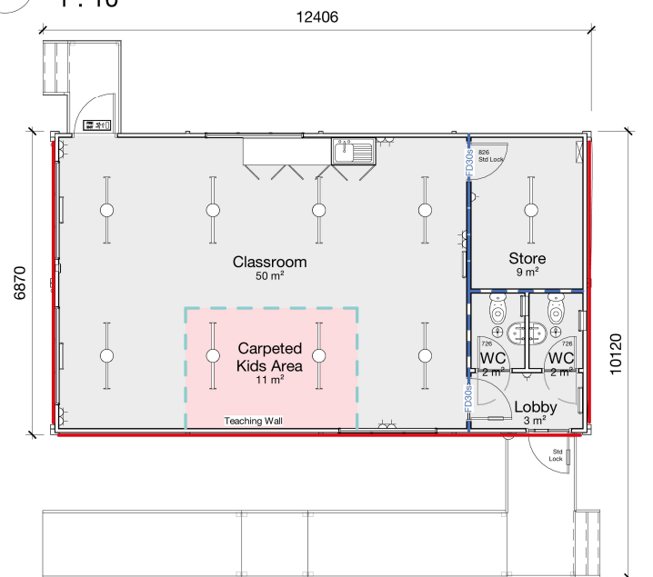
1 Proposed Layout 1 : 10
