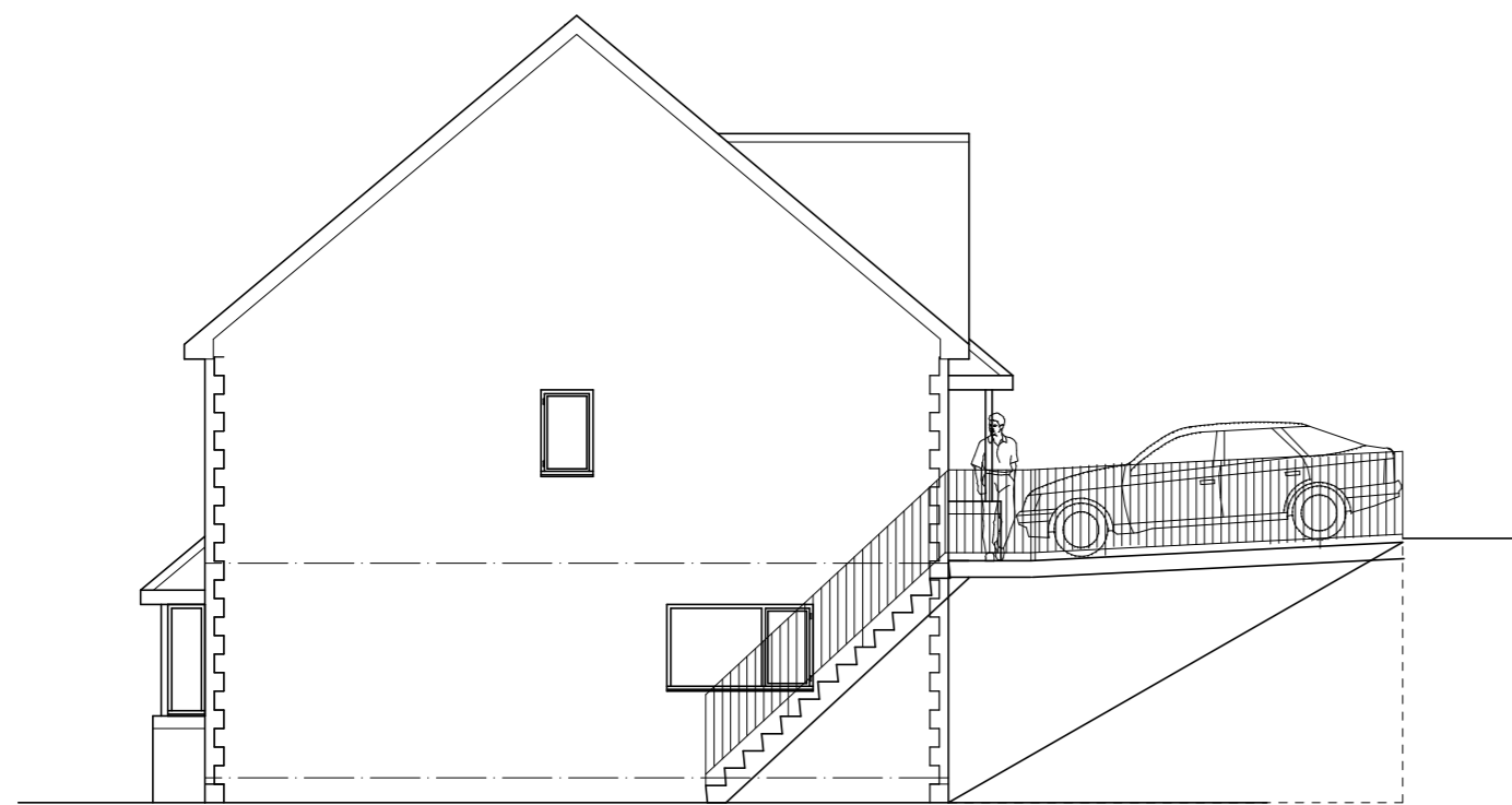
SIDE ELEVATION
