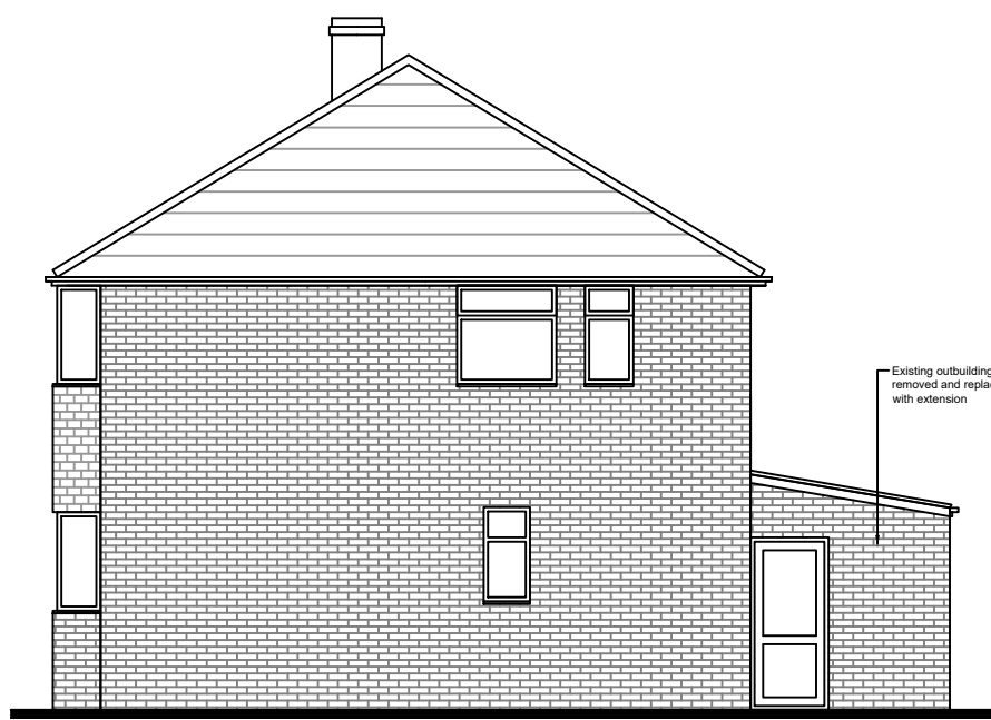
Existing Side Elevation (North Facing)
