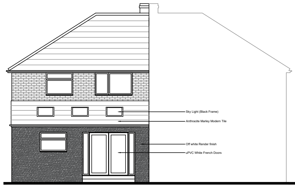
Proposed Rear Elevation (West Facing)
