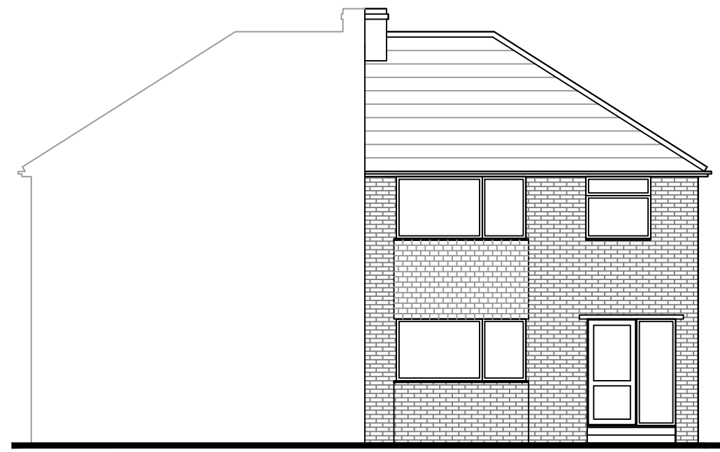
Proposed Front Elevation (East Facing)
