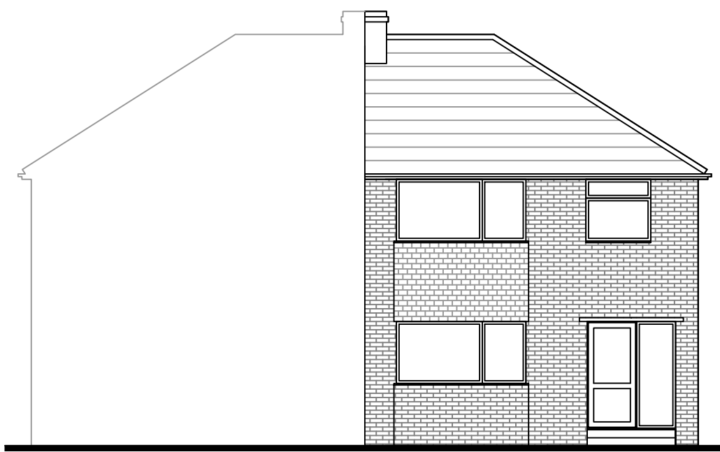
Existing Front Elevation (East Facing)
