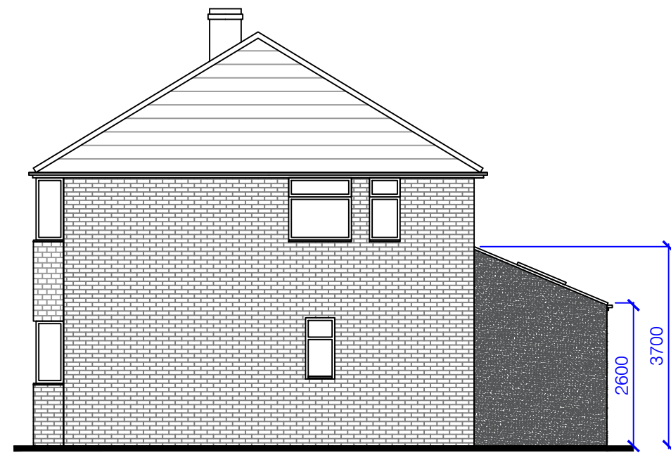
Proposed Side Elevation (North Facing)
