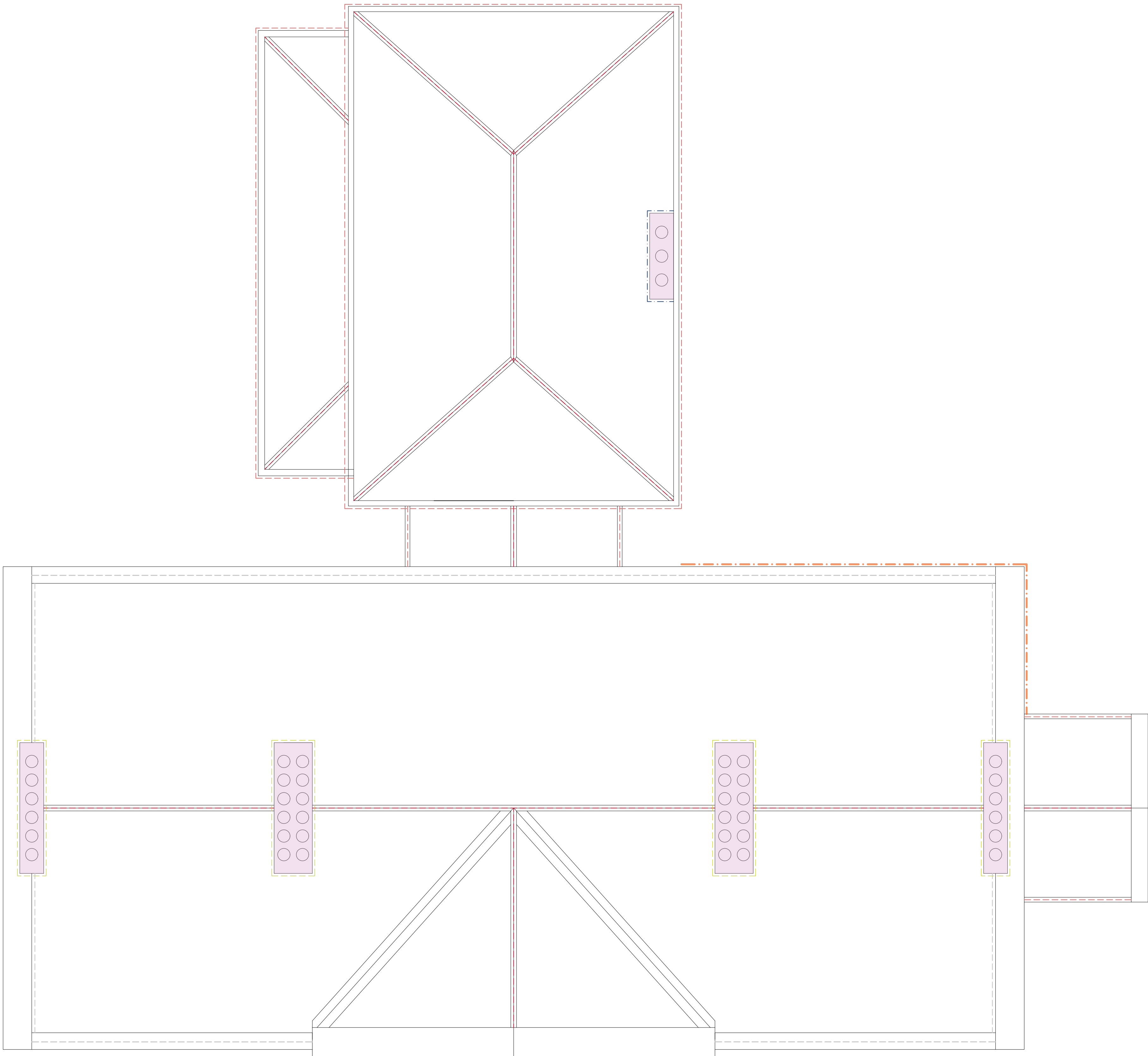
ROOF PLAN
