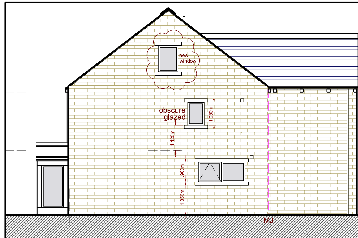
Dwelling 1 South Elevation - Proposed
