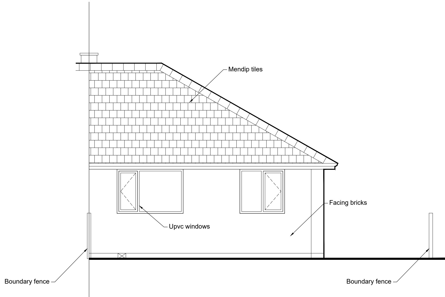
Existing Rear Elevation 1:50
