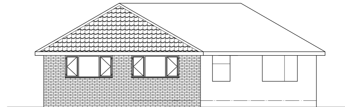
REAR ELEVATION
