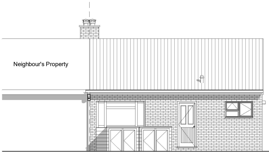
2 Proposed Rear 1 : 100
