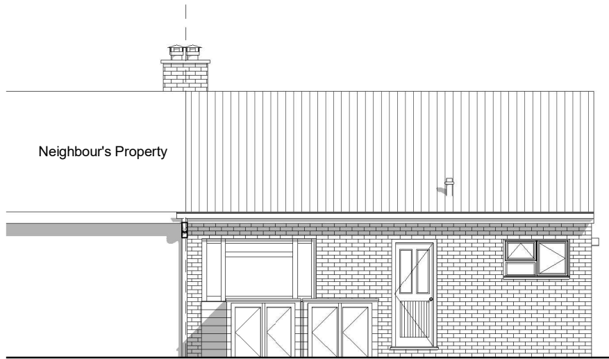
1 Existing Rear 1 : 100
