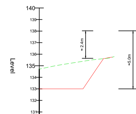
ALIGNMENT - SECTION LINE1 - LONGSECTION SCALE: H 1:500,V 1:100. DATUM: 130.000
