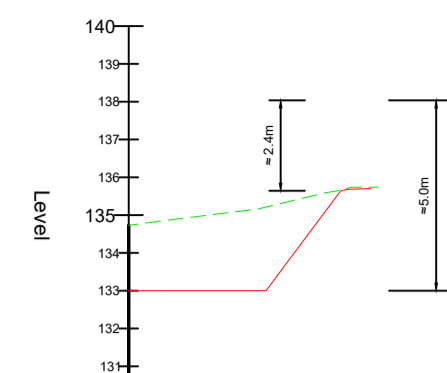
ALIGNMENT - SECTION LINE2 - LONGSECTION SCALE: H 1:500,V 1:100. DATUM: 130.000
