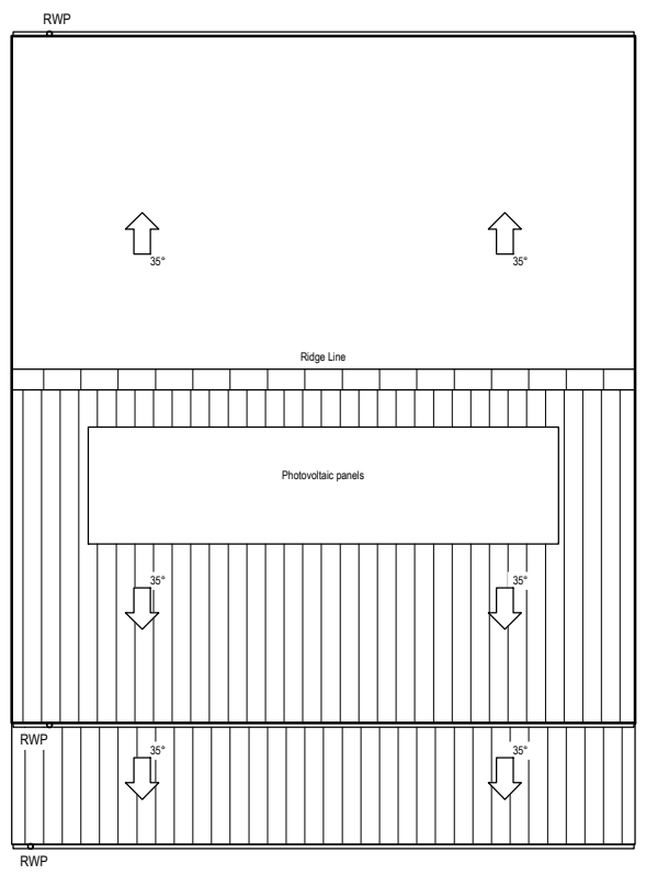
ROOF PLAN
