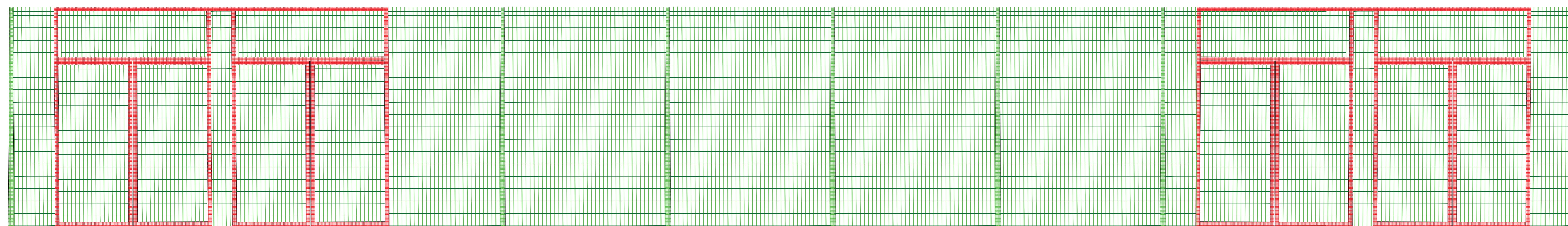
FENCE ELEVATION (FRONT) WITH ELEVATION 8 BEHIND 1:20 DOORS SHOWN RED FOR REFERENCE ONLY - TO BE GREEN RAL 6005
