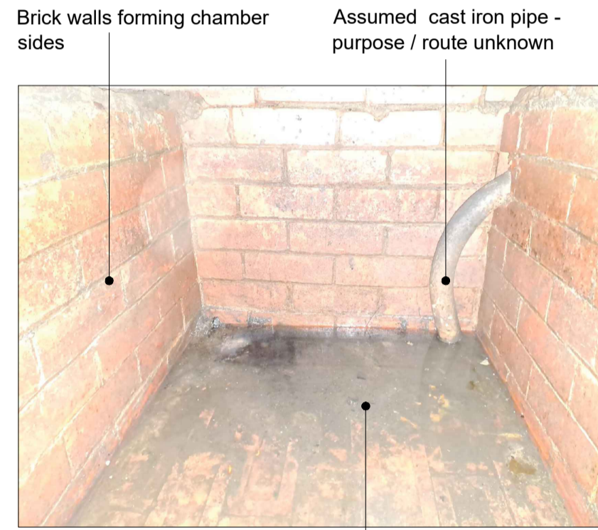
Base of sump chamber formed in brickwork
