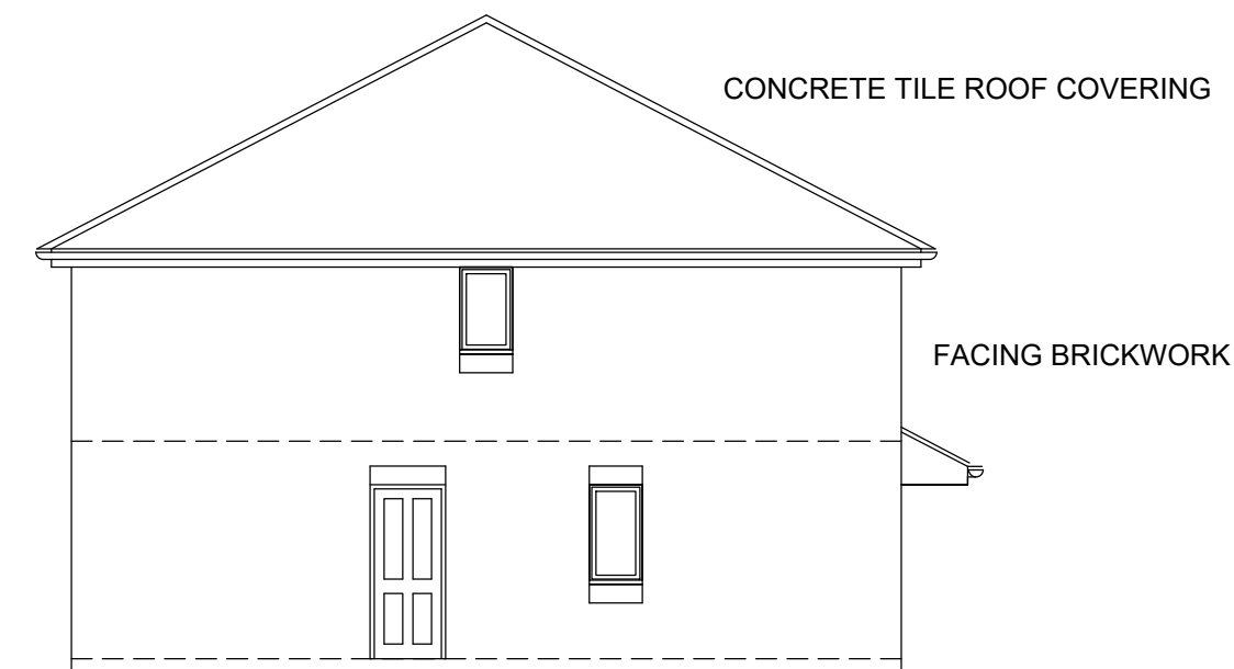
SIDE ELEVATION LEFT
