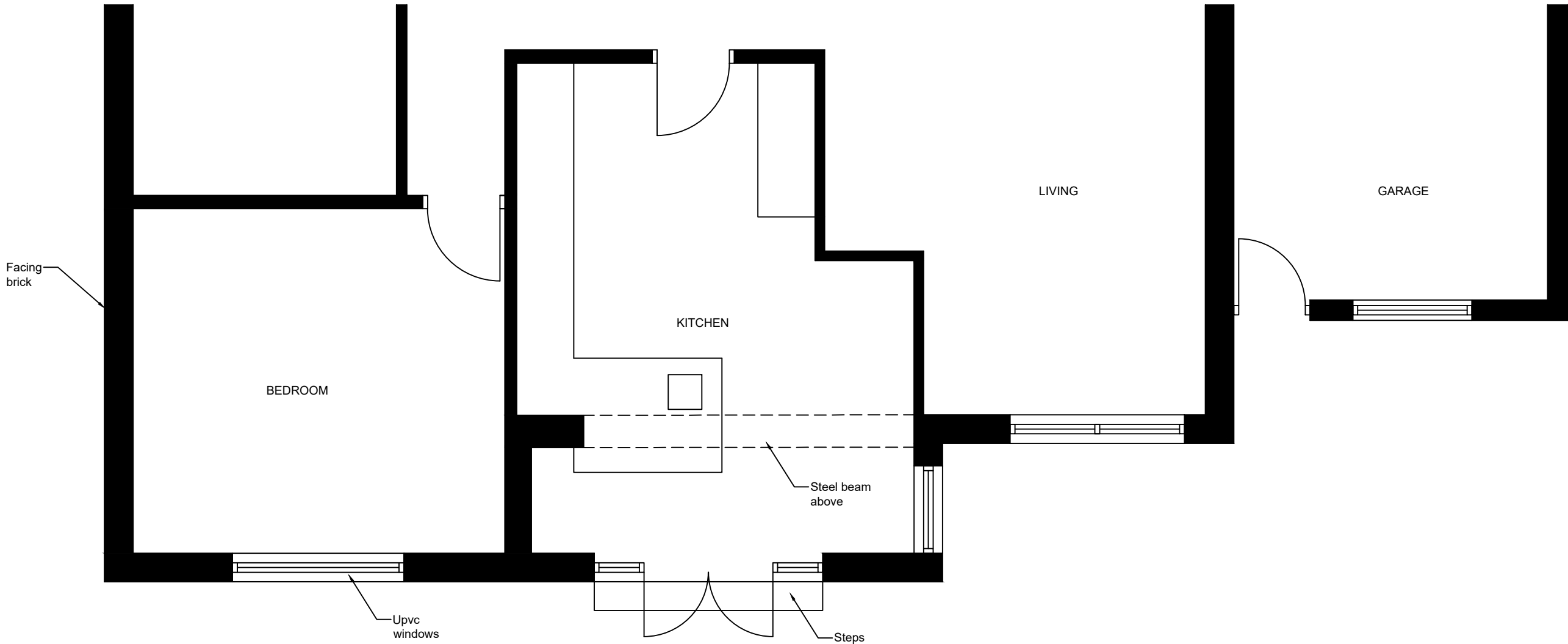
EXISTING PLAN 1:50
