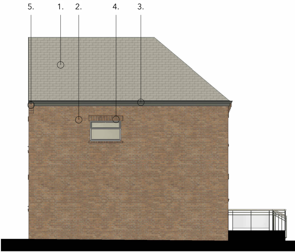
East Elevation 1 : 100
