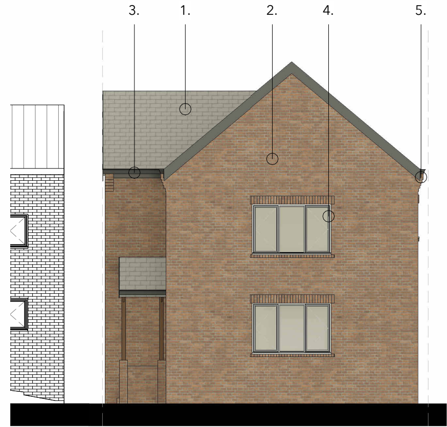
South Elevation 1 : 100
