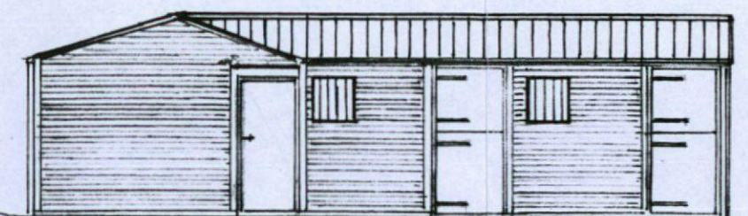
EAST ELEVATION
