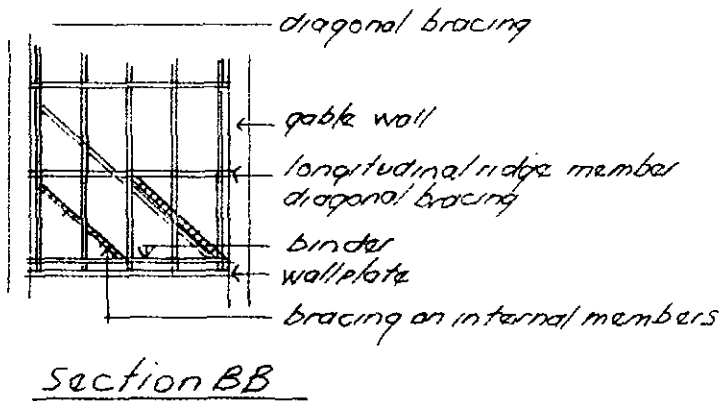
Standard Bracing For Fink Trusses
