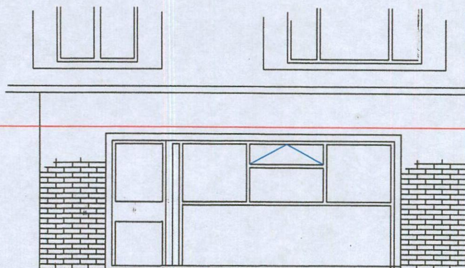
PROPOSED FRONT ELEVATION uPVC Standard Door/Window unit with solid panels to bottom of both door and window.
