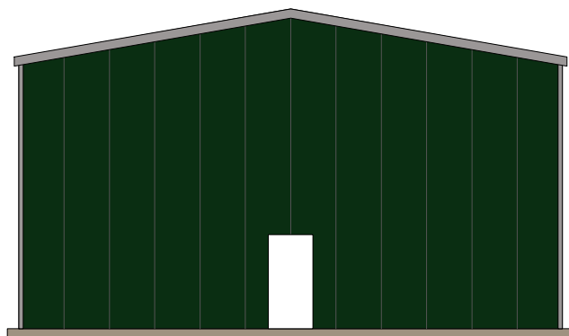
Back Elevation (Scale = 1:150)
