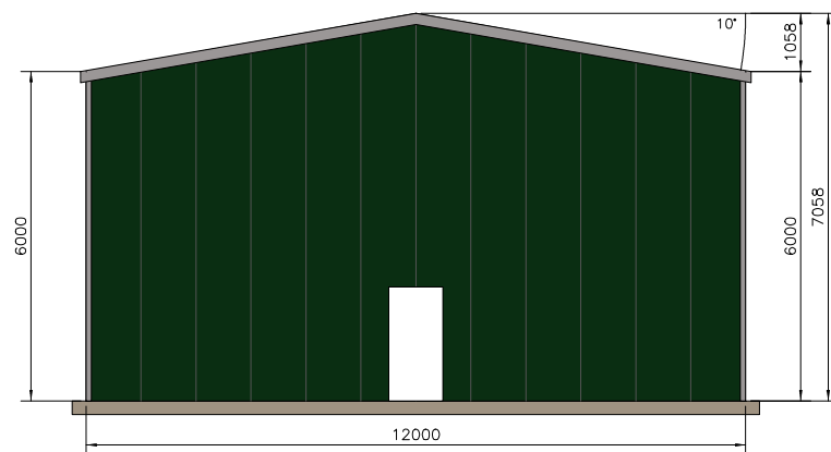
Front Elevation (External)
