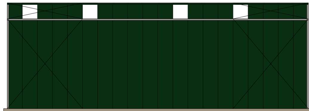
Right Elevation (Scale = 1:150)
