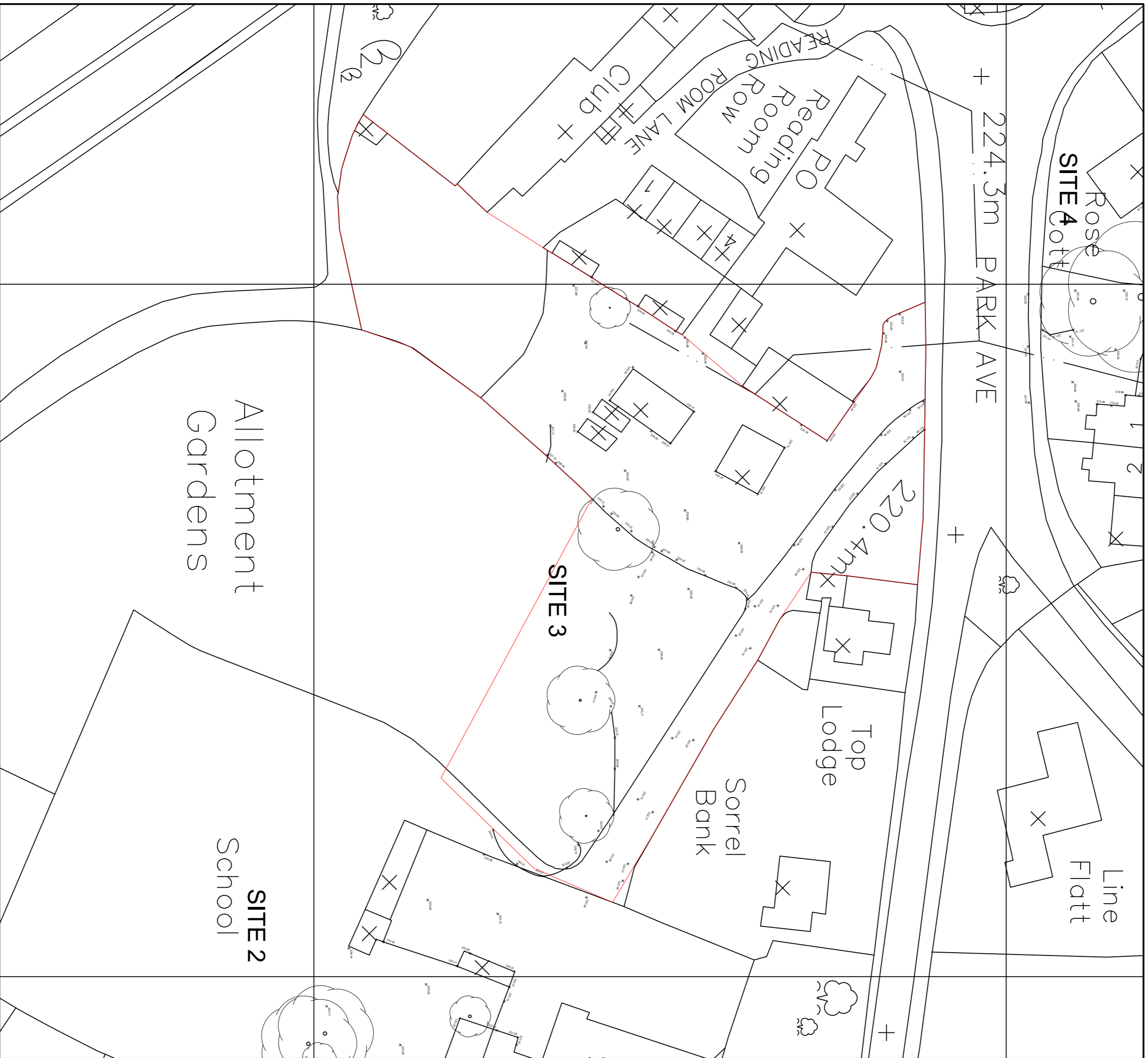
SITE AS EXISTING 1:200
