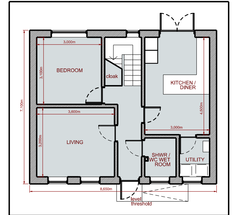
Ground Floor Plan - Proposed 1:100 No 5
