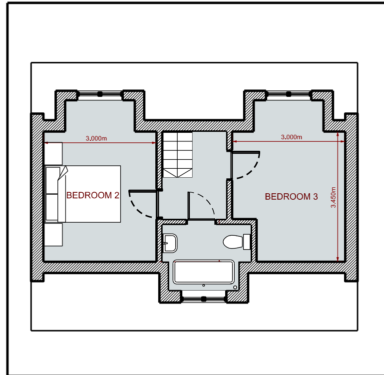
First Floor Plan - Proposed 1:100 No1,2,3,4
