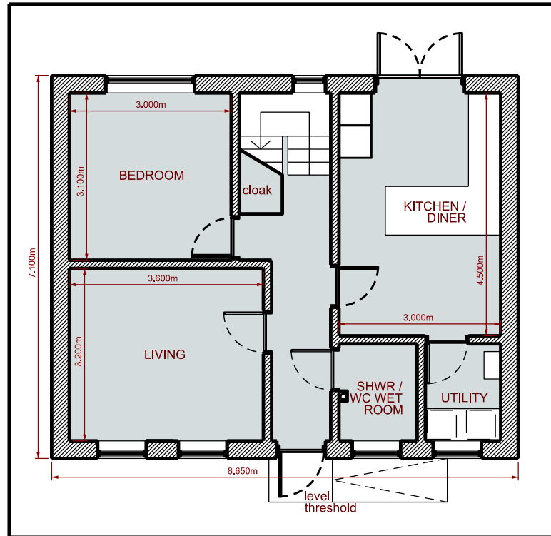
Ground Floor Plan - Proposed 1:100 No1,2,3,4
