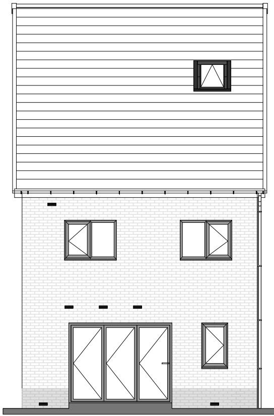
REAR ELEVATION
