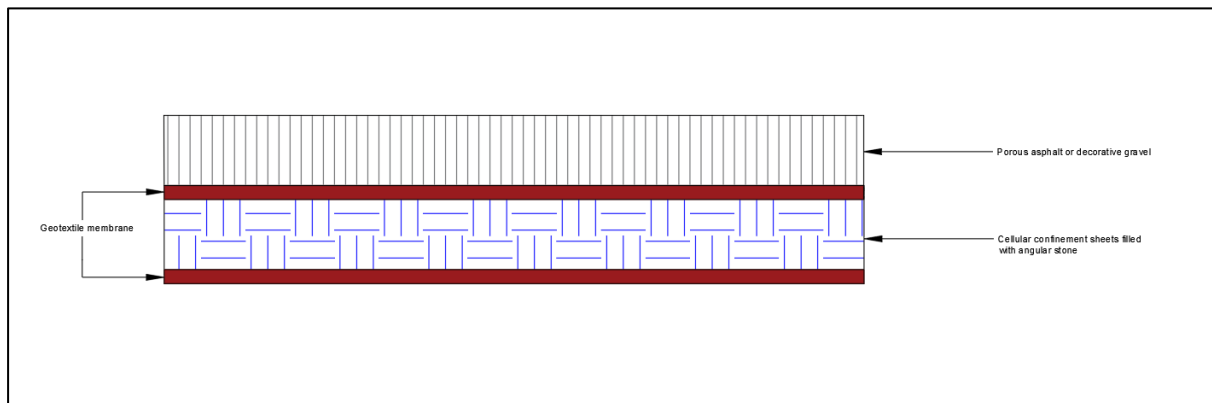
Figure 2. Cellular confinement construction
