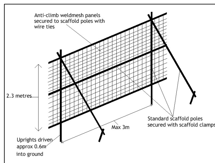
Figure 1. Temporary Protective Fencing
