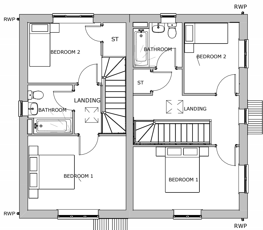
First Floor 1 : 100
