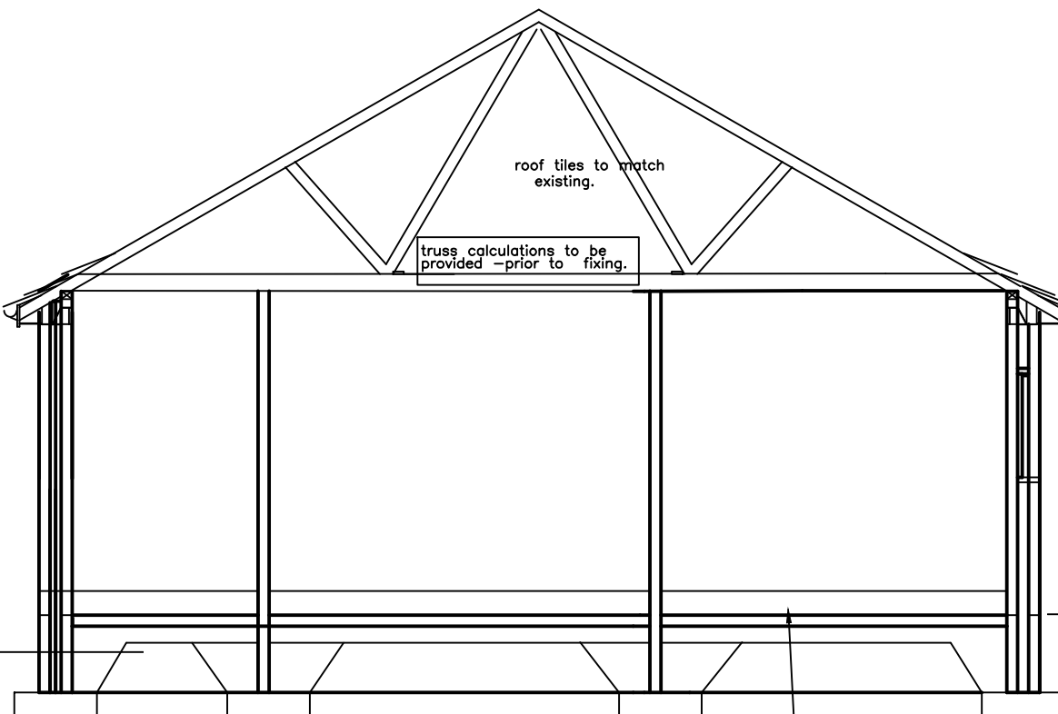
SECTION (typical)
