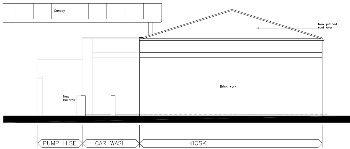
SIDE ELEVATION TO BARNESLEY ROAD AS PROPOSED
