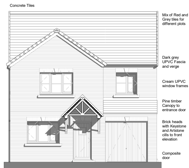
Front Elevation 1 : 100
