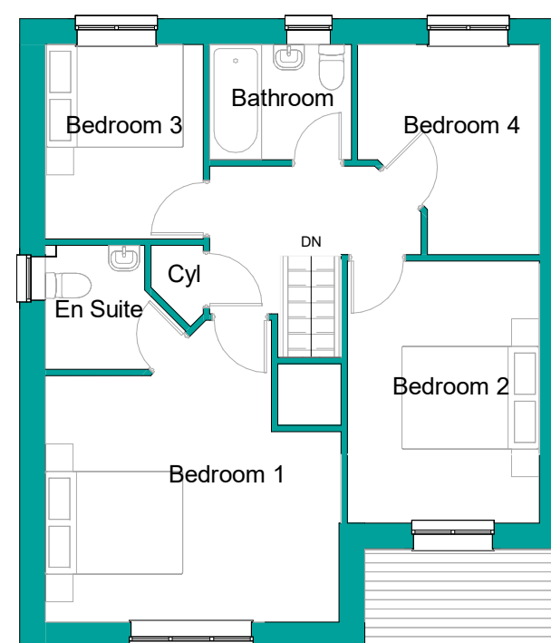
First Floor G.A. 1 : 100
