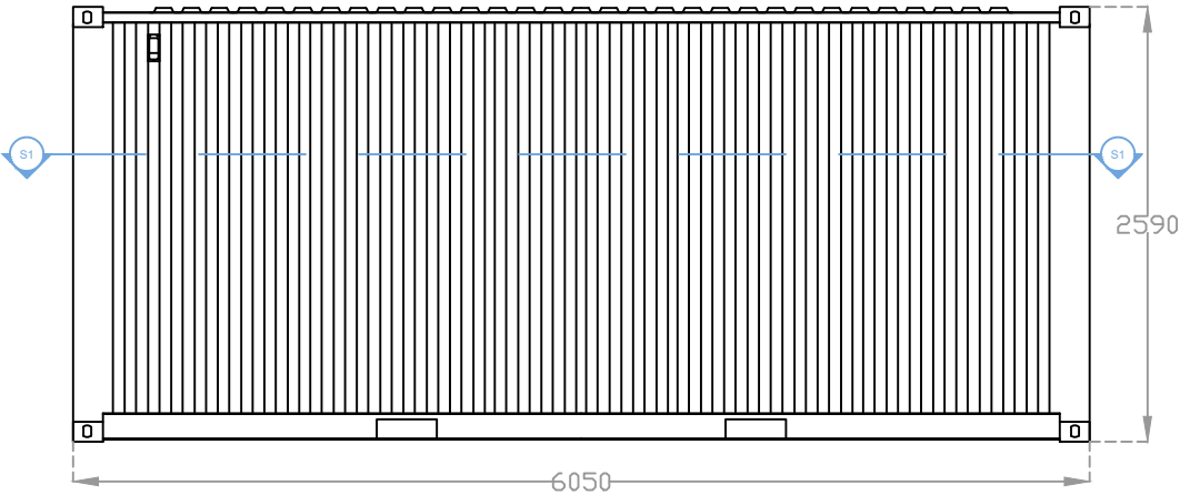
Side Elevation D
