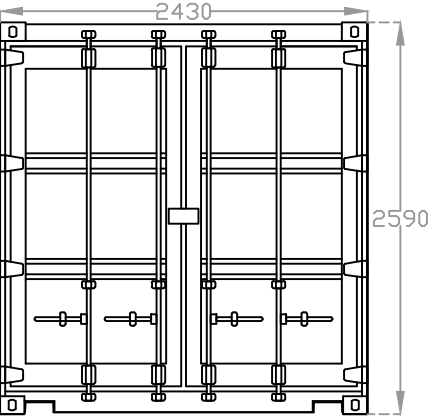
Side Elevation B (Front)
