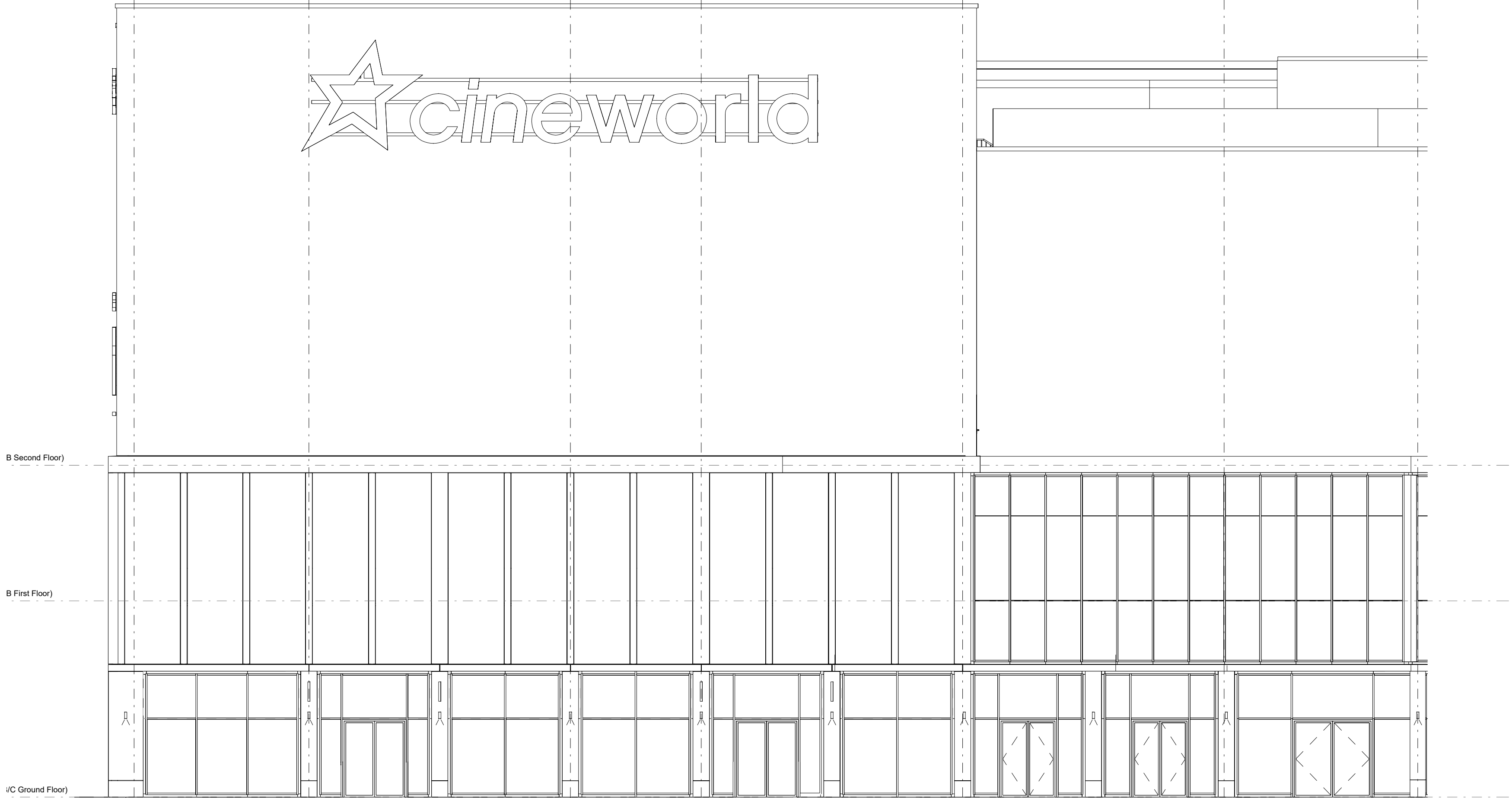
Existing West Side Elevation, 1:100
