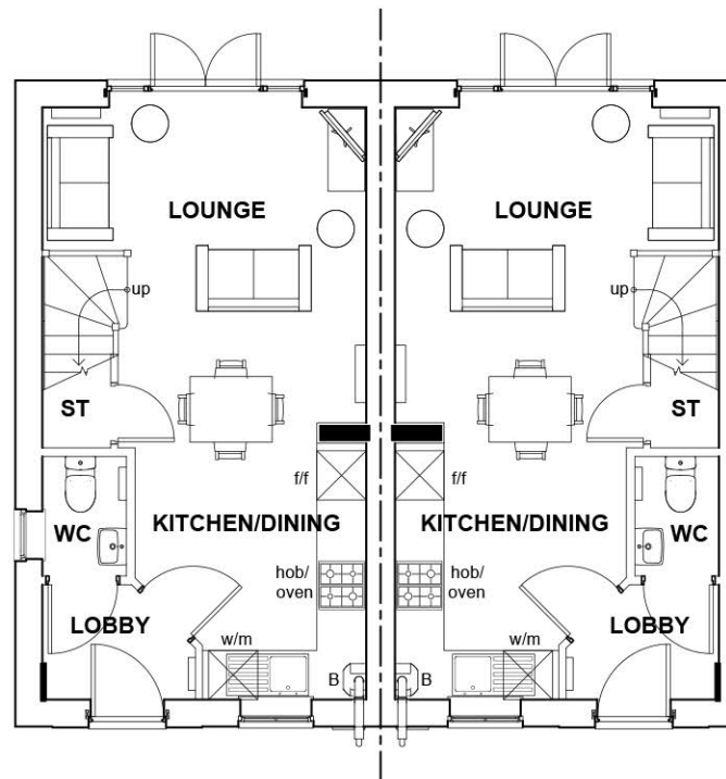
GROUND FLOOR PLAN Denford - End Denford - Mid
