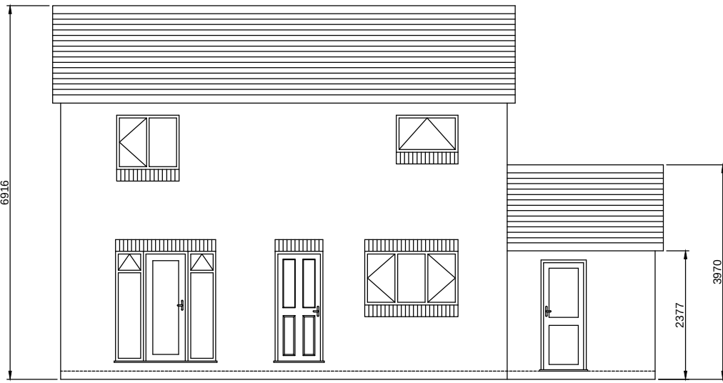
REAR ELEVATION - EXISTING
