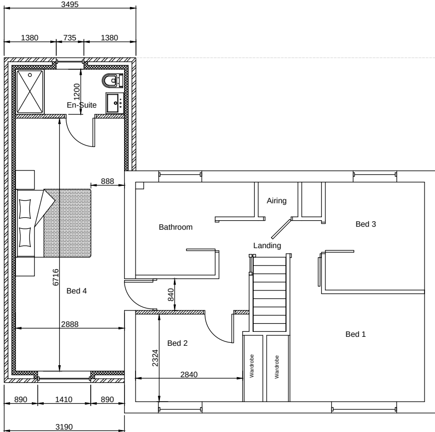
FIRST FLOOR - PROPOSED
