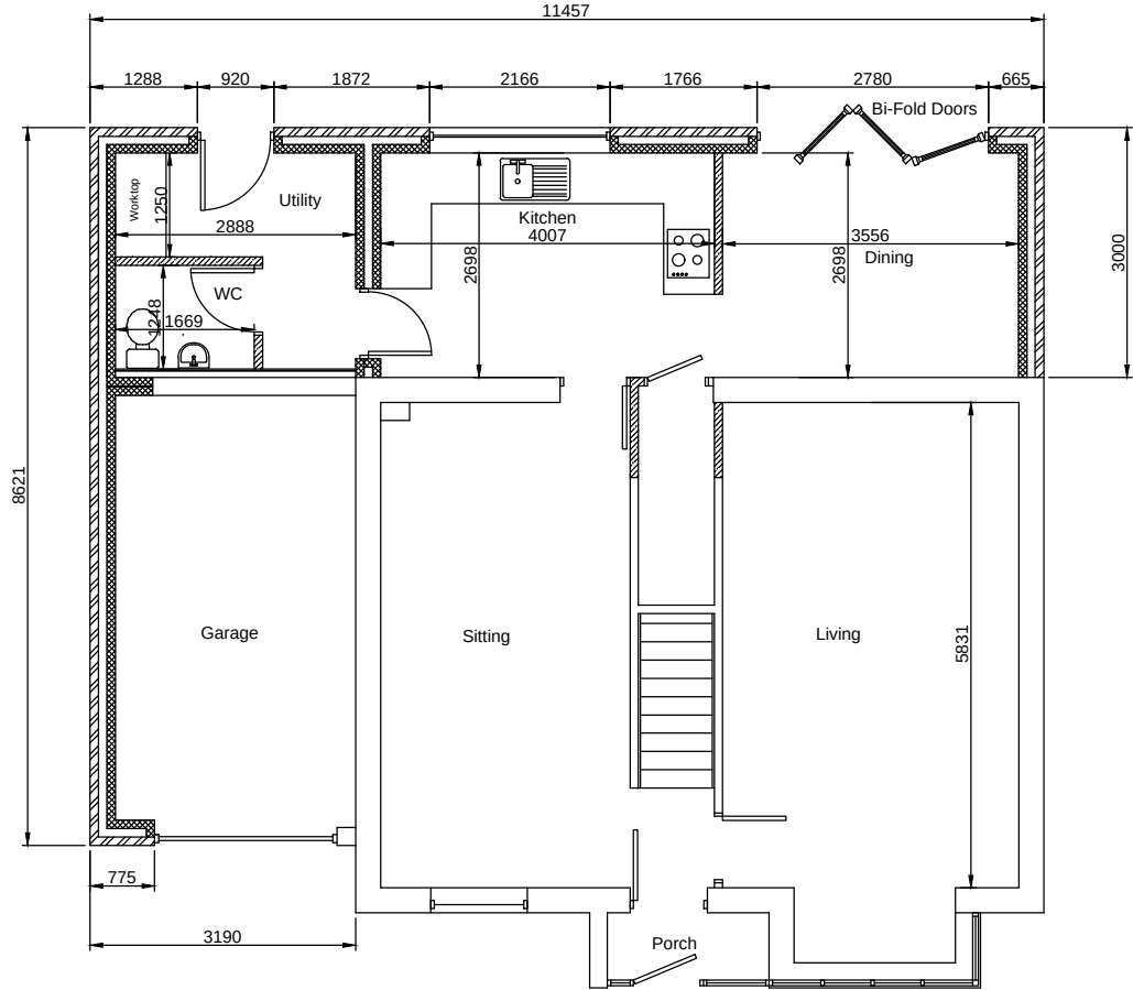
GROUND FLOOR - PROPOSED
