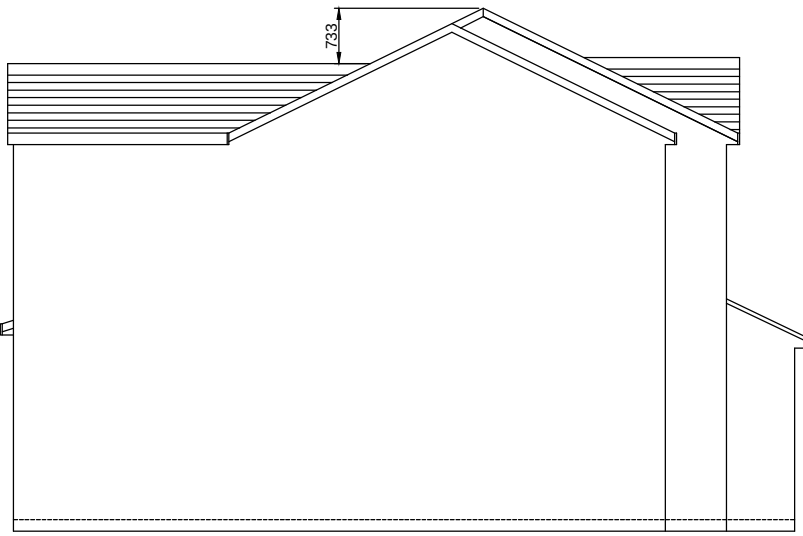
LEFT ELEVATION - PROPOSED
