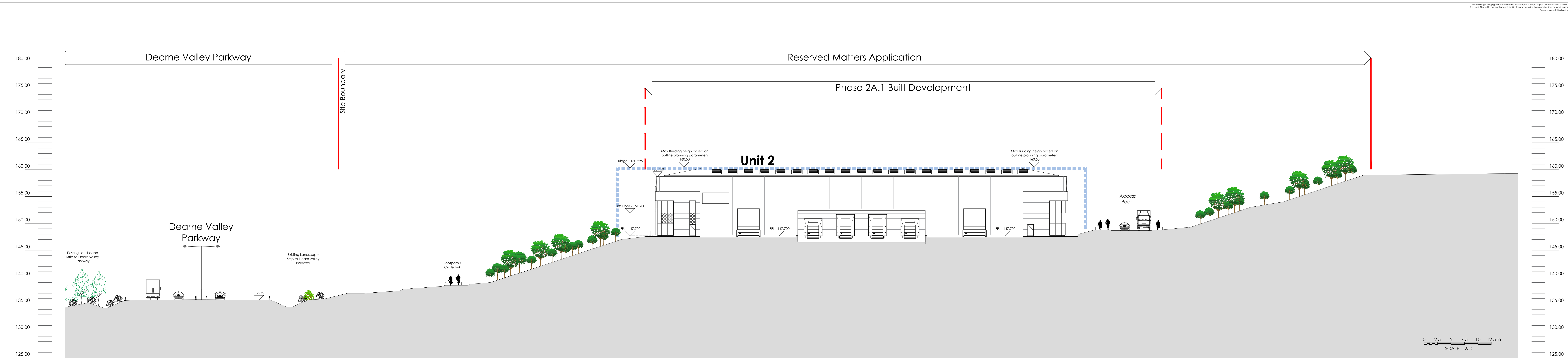
Section 2- After completion of the development - 1:500
