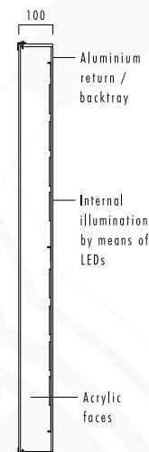
ARCH SECTION THROUGH Scale - 1:20
