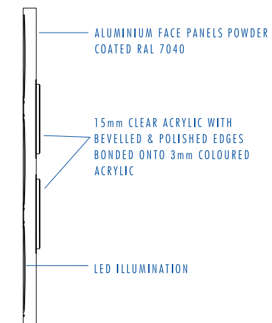
SECTION THROUGH SIGN A Scale 1:20
