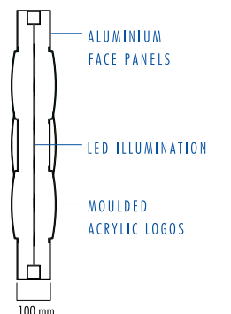
SECTION THROUGH SIGN B scale 1:20
