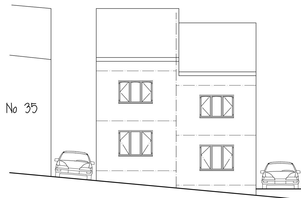
REAR ELEVATION
