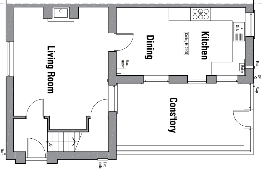
Ground Floor 1:50
