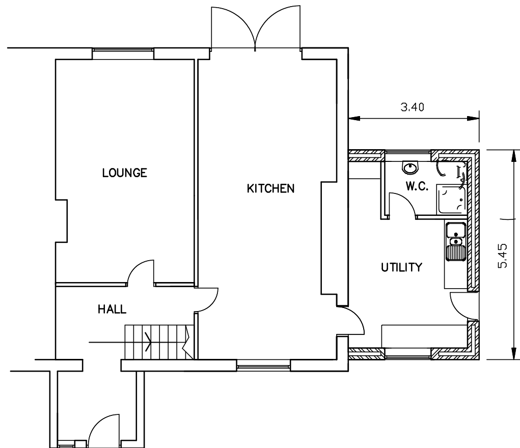
GROUND FLOOR
