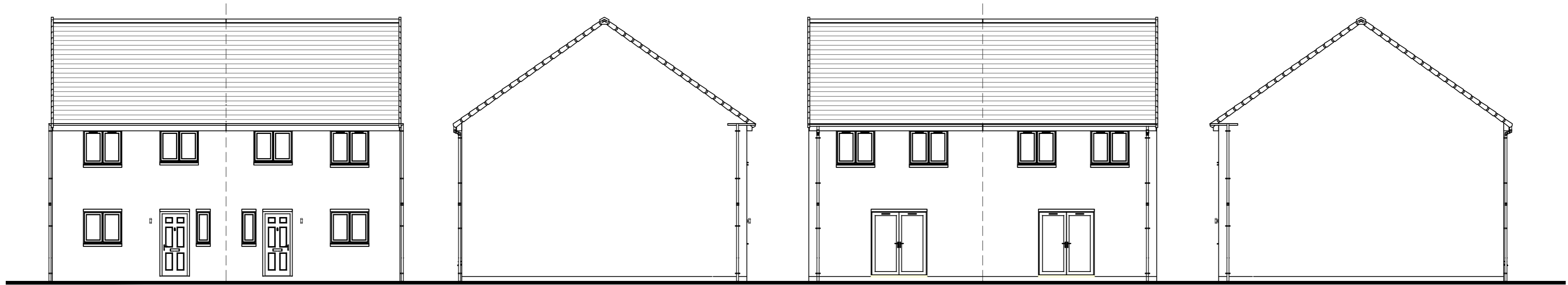
FRONT ELEVATION
