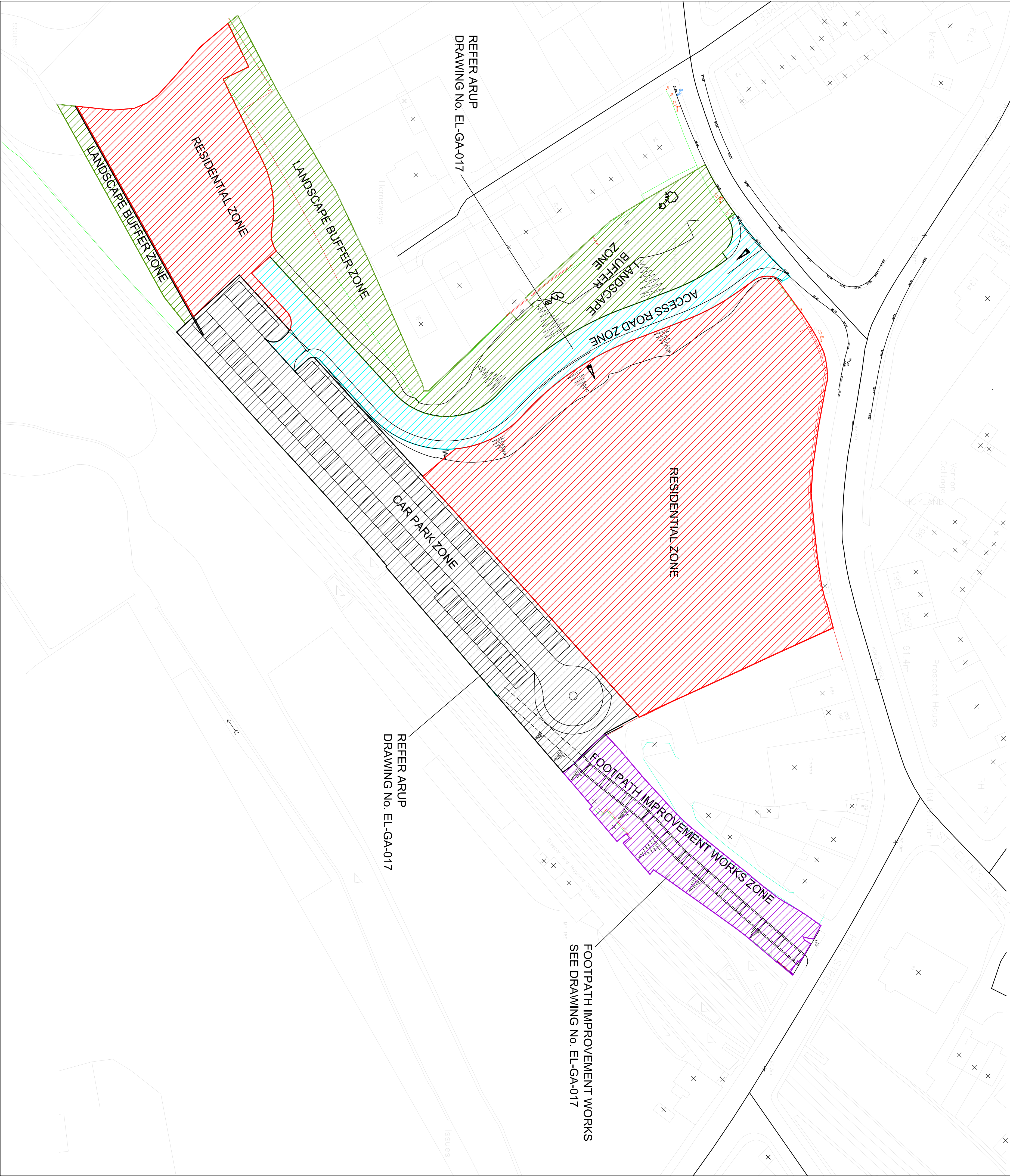
PROPOSED SITE LAYOUT 1:500 @ A1
