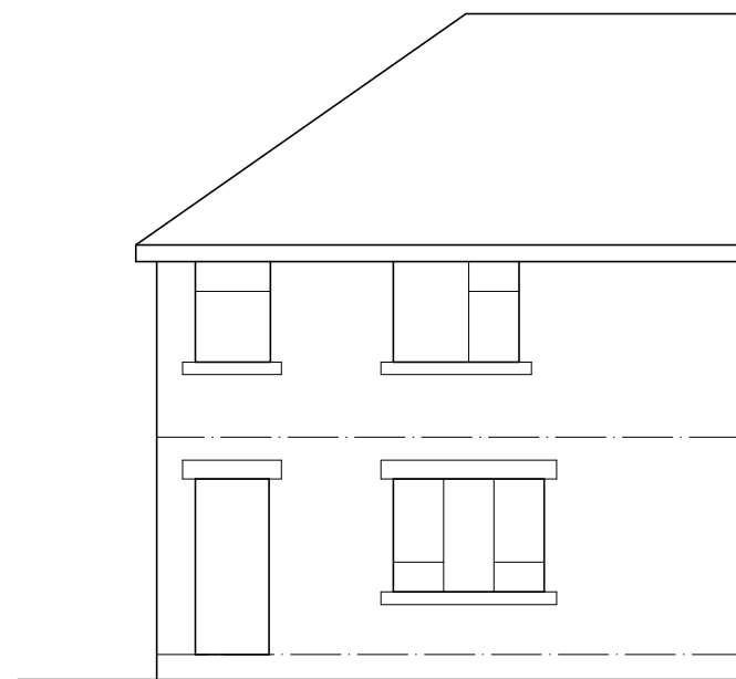
FRONT ELEVATION
