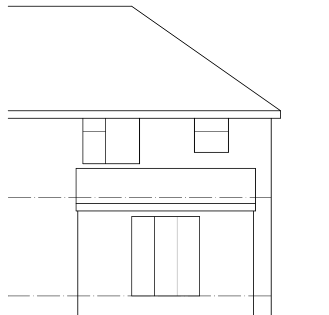
REAR ELEVATION
