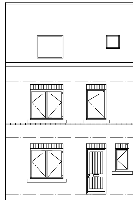
FRONT ELEVATION
